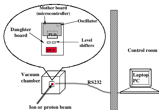
Figure 3: Measurement setup for the heavy ion irradiation. For the proton irradiation, the test board was not installed in a vacuum chamber, but in air.
