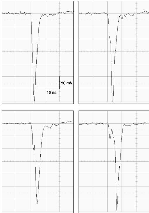
Figure 2: RPC pulse shape examples
