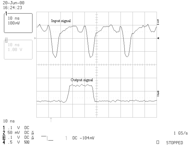
Figure 8: illustration of the “oneshot” protection.
