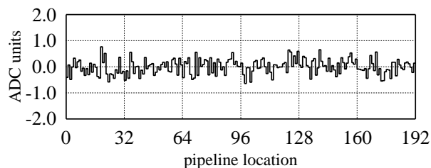
Figure 8. APV25s1 pipeline pedestals for a typical channel
