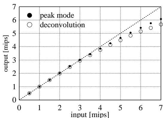
Figure 5. APV25s1 linearity
