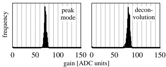
Figure 15. Gain histograms for good probed APV25s0 chips
