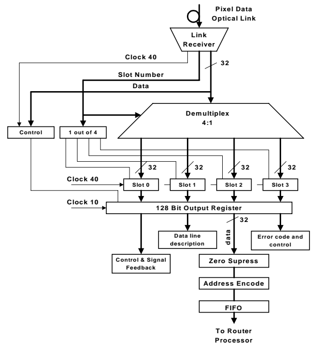
Figure 10 shows the Pixel Router receiver block diagram.
