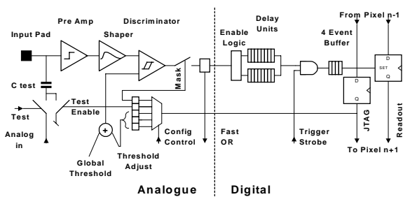
Figure 2 shows the Block Diagram of a Pixel Cell.
