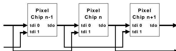
Figure 4 shows the tdi/tdo Interconnections between the Pixel Chips .
