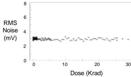
Figure 4: Noise of the Buckeye ASIC versus dose.
