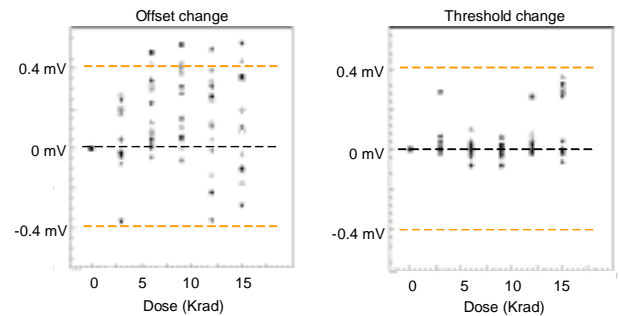
Figure 7: Changes in discriminator thresholds and comparator offsets versus radiation dose.
