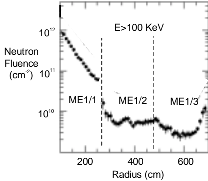
Figure 2: Neutron Fluence (for 10 LHC year) in CSC station 1.
