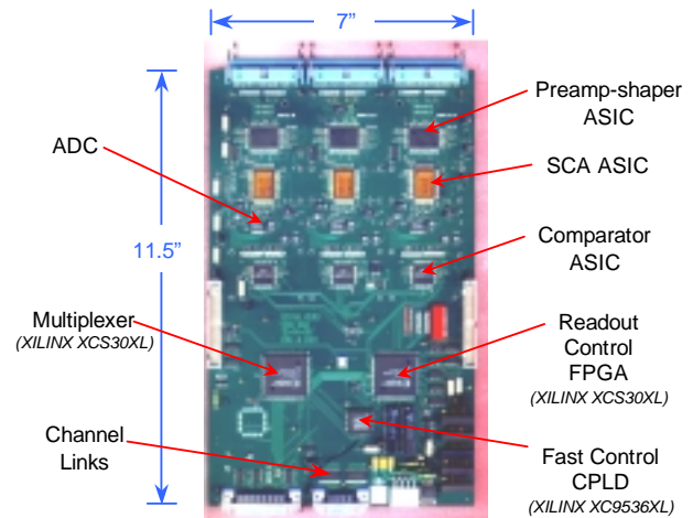
Figure 1: The CSC Cathode Front-end Board Prototype CFEB-99
