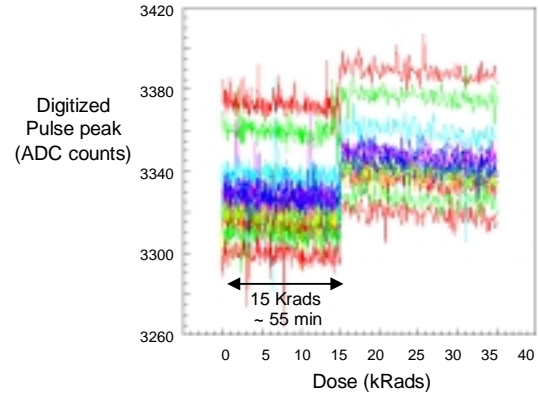
Figure 6: Performance of the SCA ASIC versus dose.
