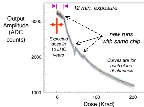
Figure 5: Gain of the amplifier-shaper ASIC versus dose.
