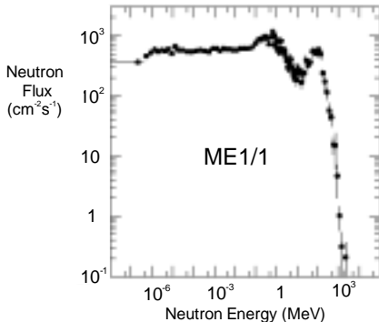
Figure 3: Neutron energy spectrum for the inner most CSC.
