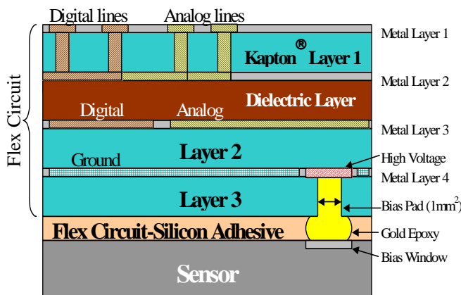
Figure 7: Sketch of Flex Circuit Cross Section
