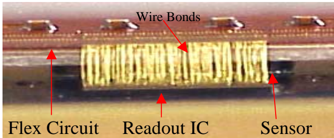
Figure 10: Pixel Module with SINTEF Sensor
