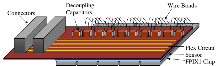
Figure 5: Sketch of the Pixel Multichip Module
