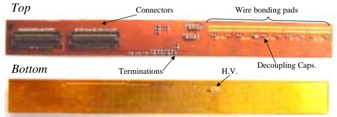
Figure 8: Flex Circuit Picture
