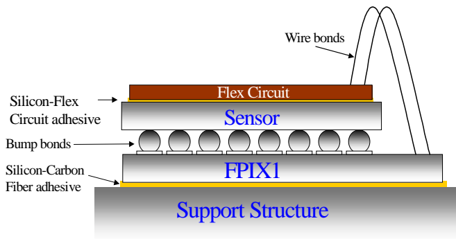
Figure 6: Sketch of the Pixel Multichip Module "Stack"
