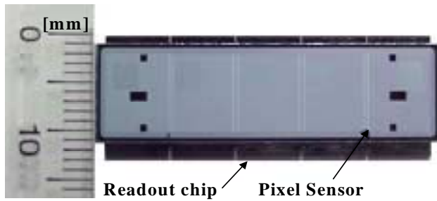
Figure 13: 5-chip Pixel Module with Indium Bumps
