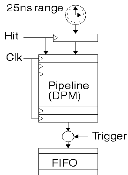
Figure 1: Pipelined TDC
