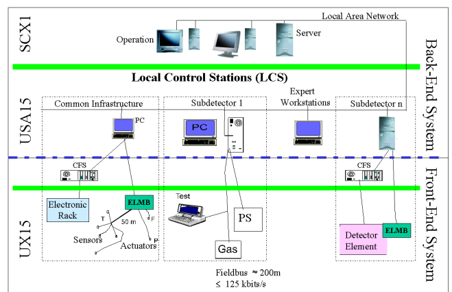
Figure 1: Architecture of ATLAS DCS
